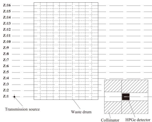
Fig.2 Side view of the TGS model.
