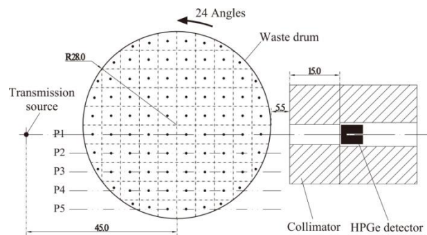
Fig.1 Vertical view of the TGS model (unit: cm).
