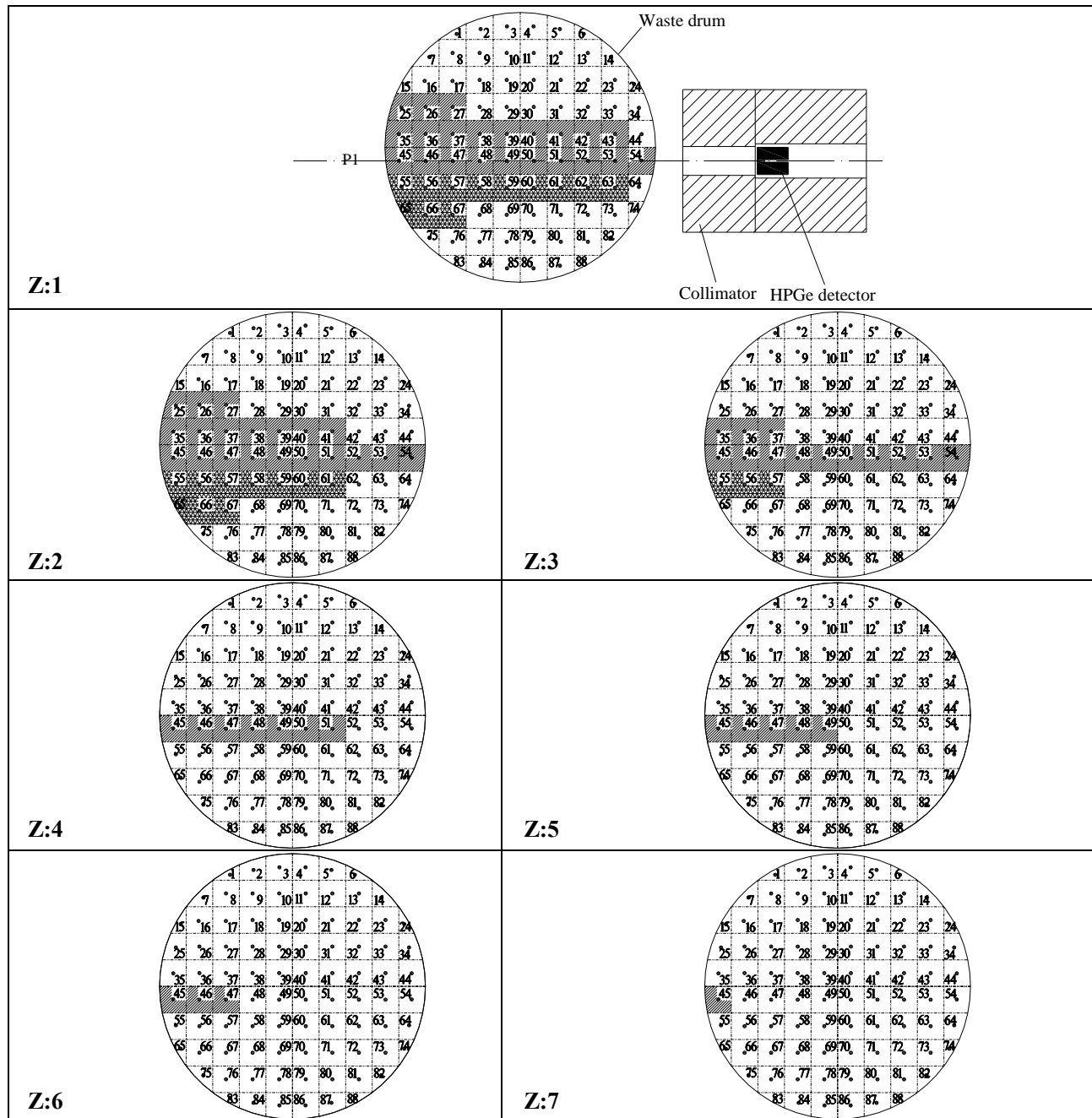
Fig.4 Point sources in FOVs at the first rotation angle 0° when emission-measuring the first layer at the P1 translation position.
