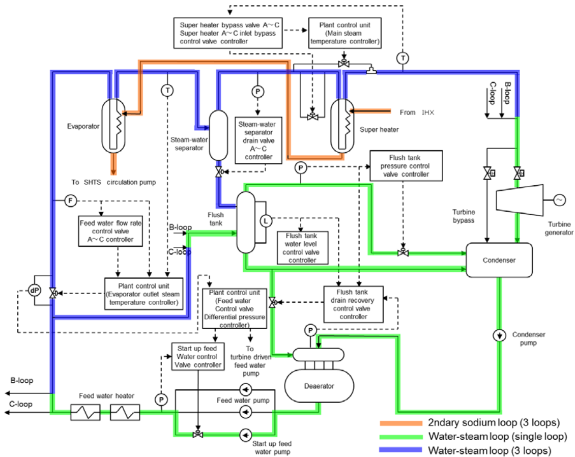
Fig. 2 Main flow paths and control systems for MONJU.
