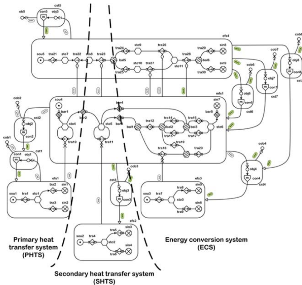
Fig. 5 MFM for superheated generation mode (sub-mode of mode B).
