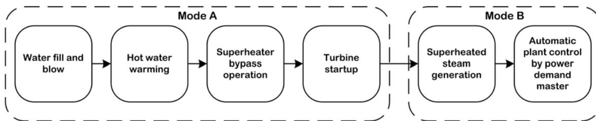
Fig. 3 Modes of the MONJU Plant startup.
