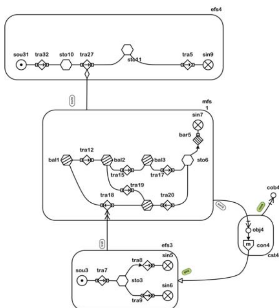
Fig. 6 MFM of the hot water warming mode (sub-mode of mode A).
