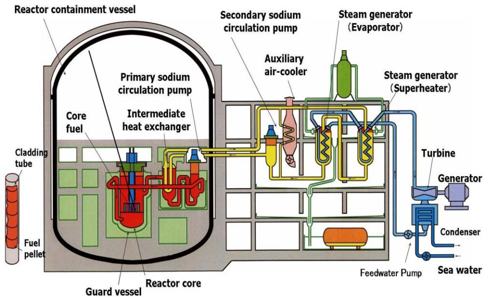
Fig. 1 MONJU plant overview.
