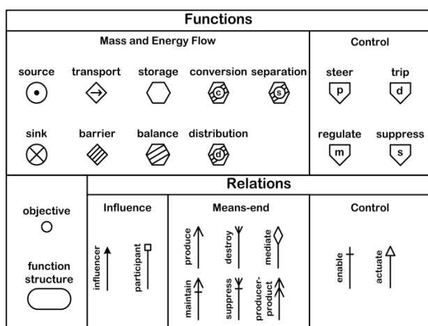
Fig. 4 MFM concepts and symbols.
