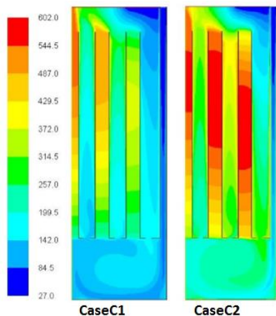
Fig. 11 Temperature distribution comparison for different wattle arrangements.
