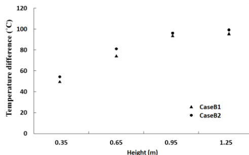
(b) Cross-sectional average temperature rise for CaseB1 and CaseB2
