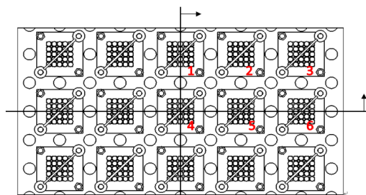
(a) The schematic of rod heater bundle identification number
