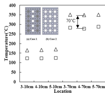
(a) Effect of backplane hole arrangement on temperature at H=30cm
