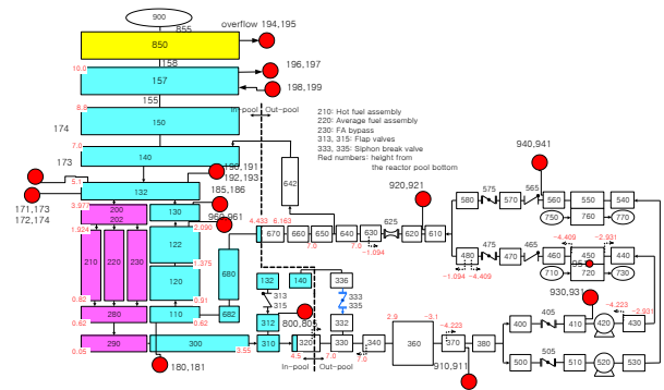
Fig. 3 MARS code nodalization for primary cooling and pool systems.
