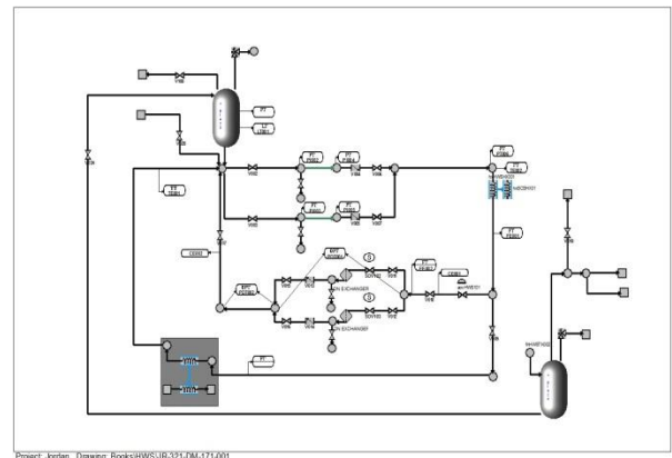
Fig. 4 Heavy water system dynamic model using 3KeyMaster.
