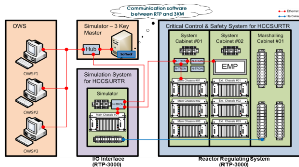
Fig. 10 Interface with simulator and controller.
