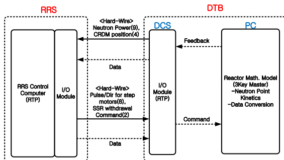
Fig. 9 Configuration of DTB test.
