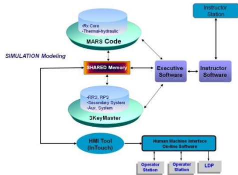
Fig. 2 HANARO simulator software configuration.
