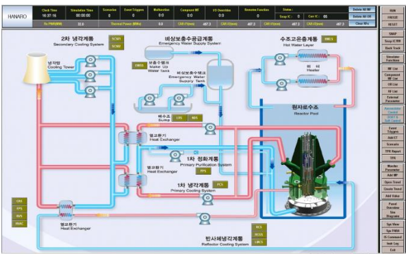
Fig. 7 Main display page of instructor station.
