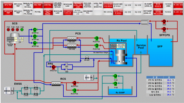
Fig. 5 Large display panel in HANARO simulator.
