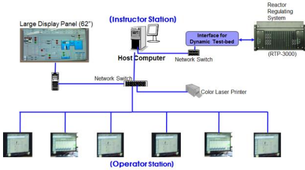
Fig. 1 HANARO simulator hardware configuration.
