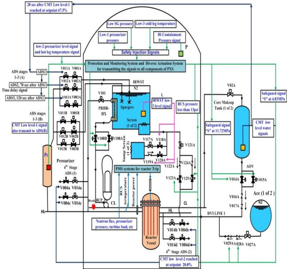
Fig. 6. Single loop model of PMS of AP1000 [7] .
