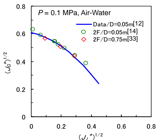
Fig.20 Effects of diameters on CCFL characteristics.
