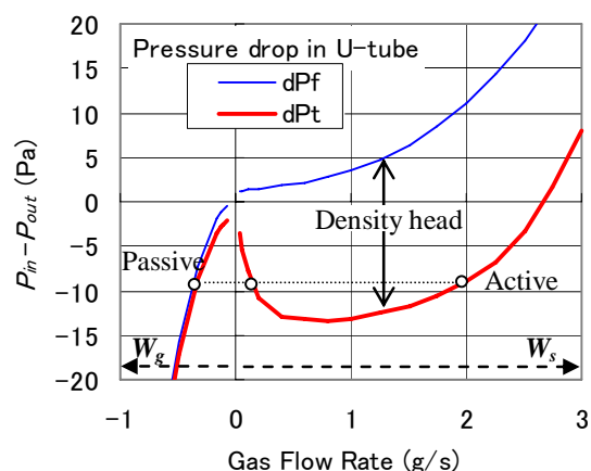
Fig.4 Pressure drop between inlet and outlet plenums in average-length U-tube. (dPf: friction loss, dPt: total pressure drop)
