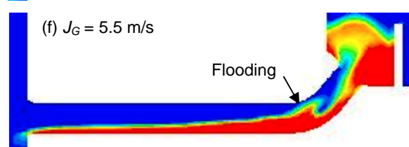
Fig.19 Observed and calculated flow patterns. ( J_{Lin} = 0.17 \text{ m/s} , Liquid fraction: see Fig. 17)
