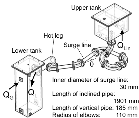
Fig.9 CCFL test apparatus in surge line.
