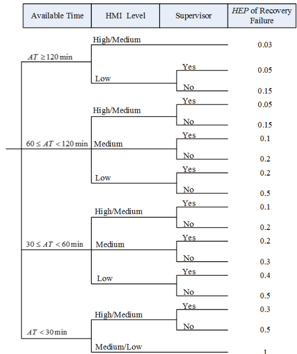
Fig. 3 Decision tree for determining the recovery failure probability of a primary task.
