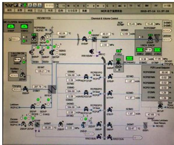
Fig. 2 Soft control screen of the RCV.
