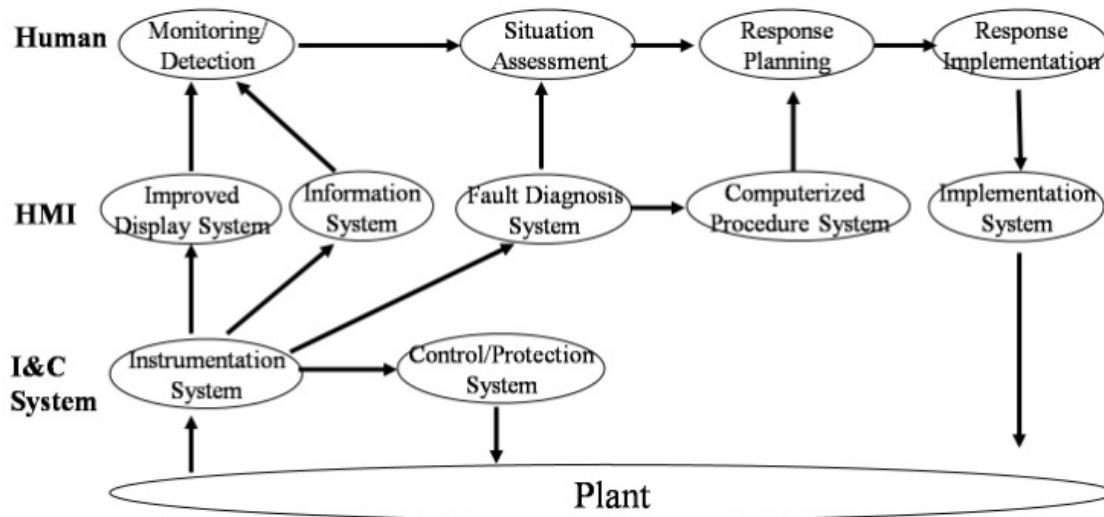
Fig.4 NPP operation process with operator support systems.
