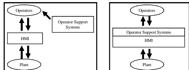
Fig.2 Independent and included operator support systems.
