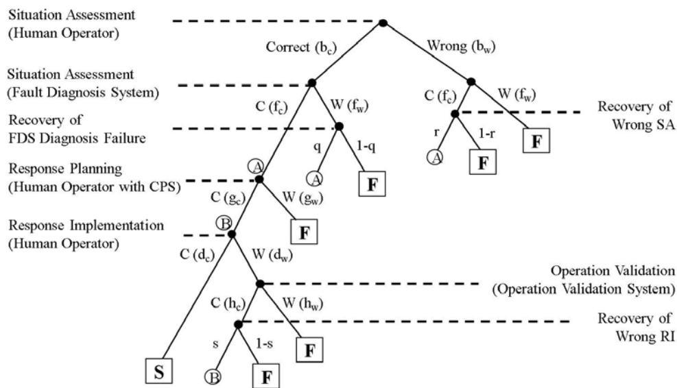
Fig.8 HRA event tree with four operator support systems.
