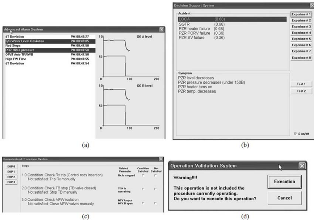
Fig.9 The prototypes of operator support systems.
