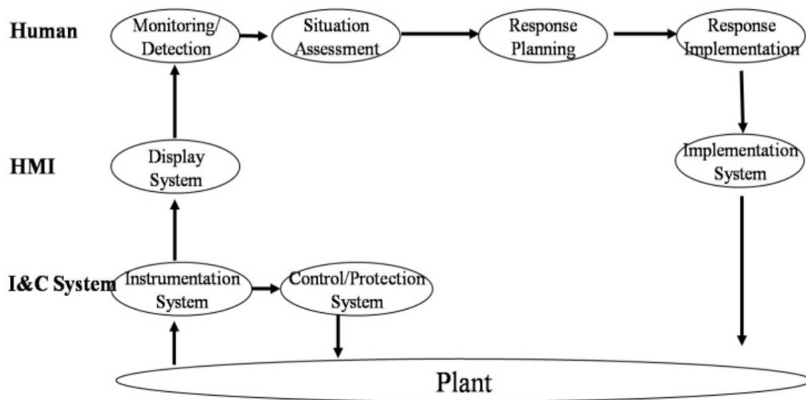
Fig.3 NPP operator’s operation process [13] .
