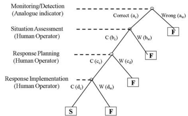
Fig.7 HRA event tree with no operator support system.
