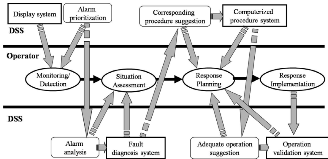
Fig.5 The architecture of INDESCO.
