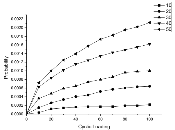
Fig.9 Probabilities in every 10 cyclic loadings under 5 different temperature differences.
