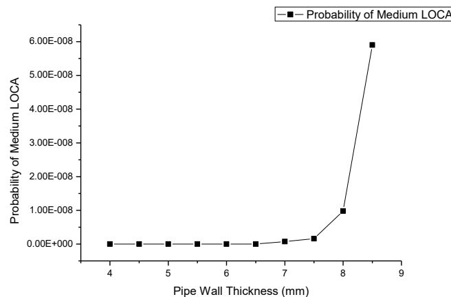
Fig.13 Probability of medium LOCA varies with wall thickness.
