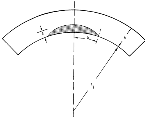
Fig.1 Crack geometry.
