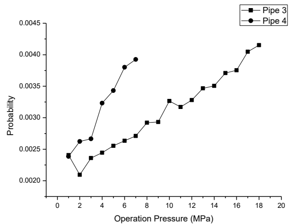
Fig.10 Break probability varies with pressure difference.
