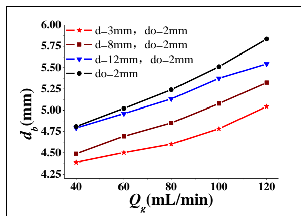
Fig.5 Bubble departure diameter.
